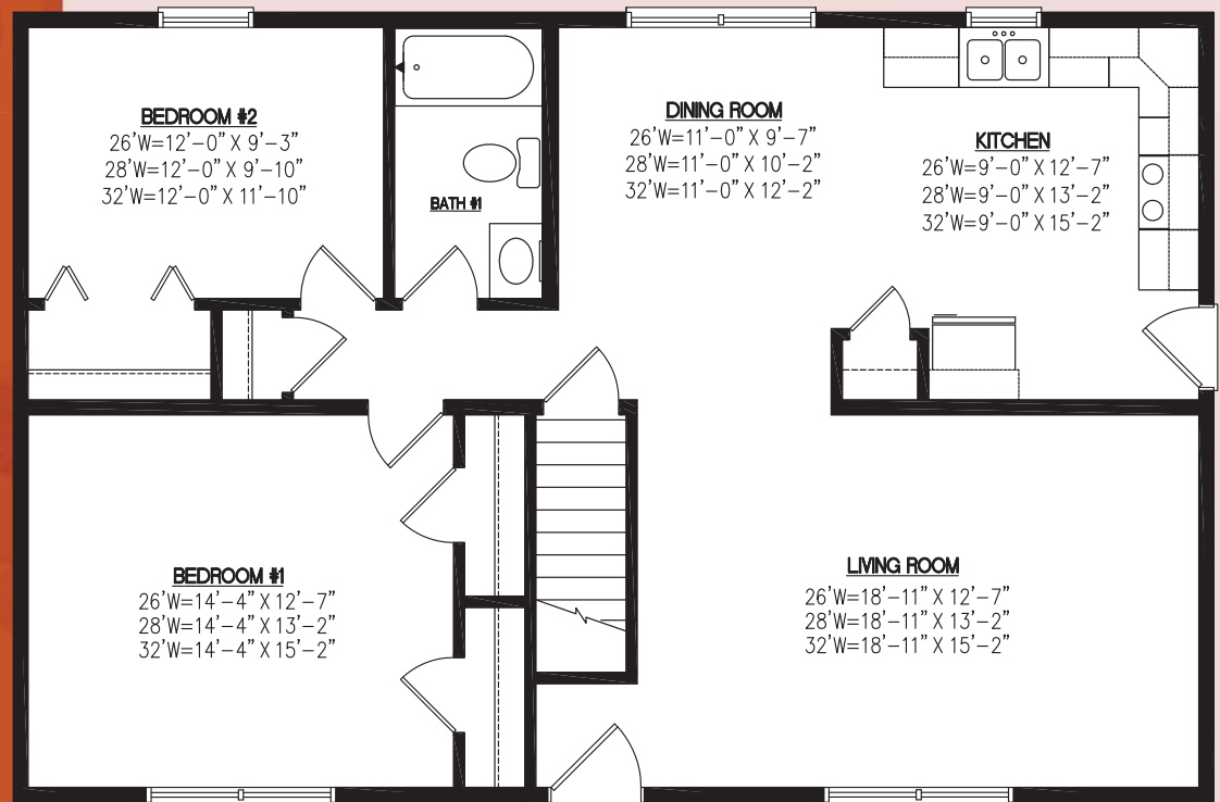
Raised-Ranch 1053 sq. ft.
