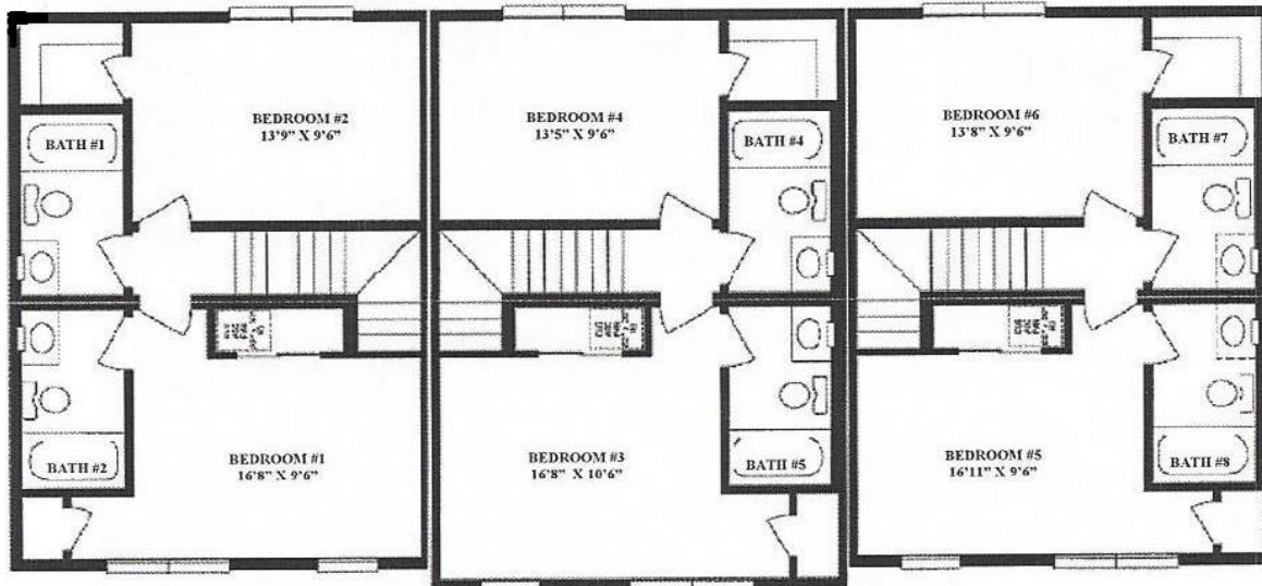
TRI-PLEX FLOOR PLAN 2 QN 11386
